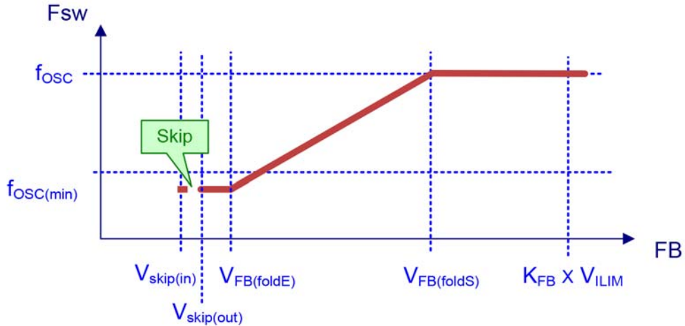
Figure 60. Frequency Foldback Mode Characteristic
