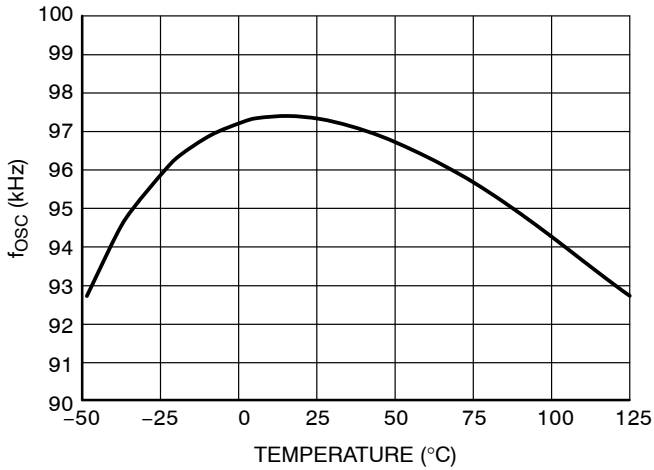
Figure 23. Oscillator f_{OSC} for the 100 kHz Version
